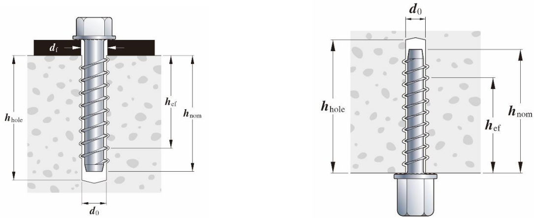
FIGURE 1—MEGABOLT HEX WASHER HEAD DETAIL (Left Picture) AND MEGABOLT HEX COUPLER HEAD INTERNALLY THREADED ANCHOR DETAIL (Right Picture)
